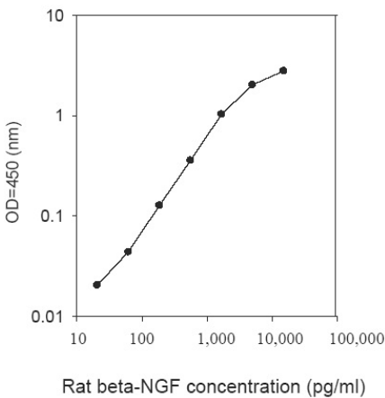
Figure 1. Example of typical rat beta NGF standard curve. The standard curve was prepared as described in Section 10.
